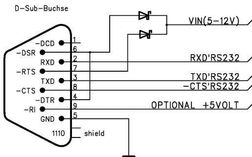
RS232 Interface
