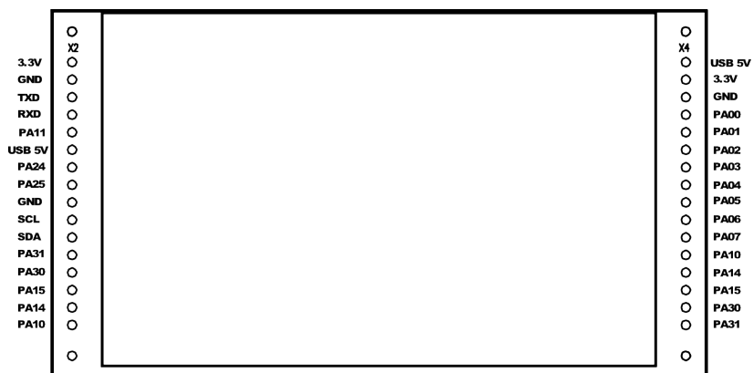
Figure 2.4. Pin-out LCDTerm35
