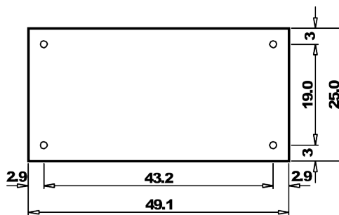
Figure 4.1. LCDTerm12 dimensions 2
