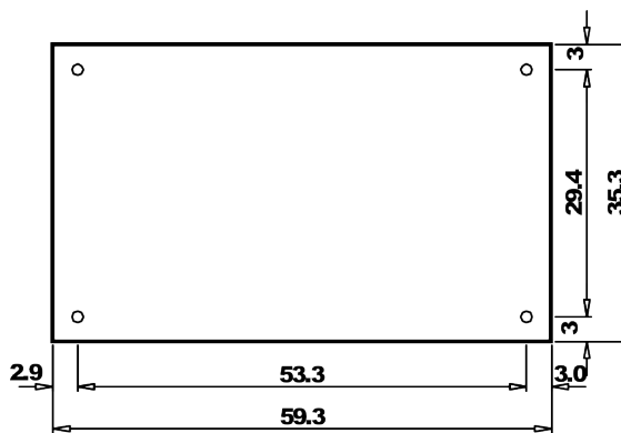
Figure 4.2. LCDTerm15 dimensions 2
