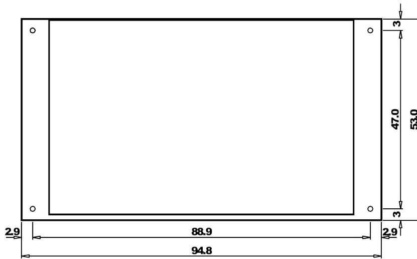
Figure 4.4. LCDTerm35 dimensions 2
